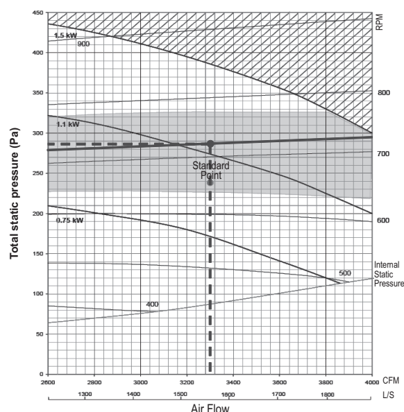
UATYQ250 - blower curve
