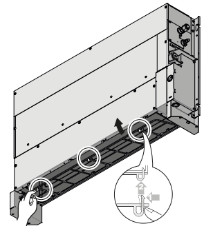
bottom suction
