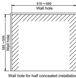
Wall hole for half concealed installation
