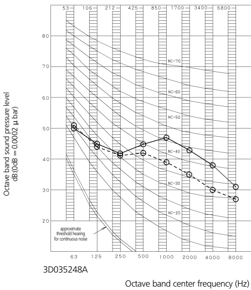
FLXS60B (Cooling)
