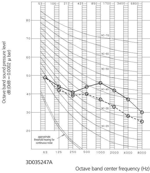
FLXS50B (Cooling)
