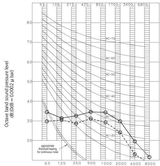
FLXS35B (Heating)
