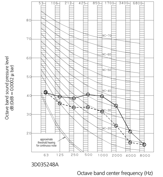
FLXS60B (Heating)
