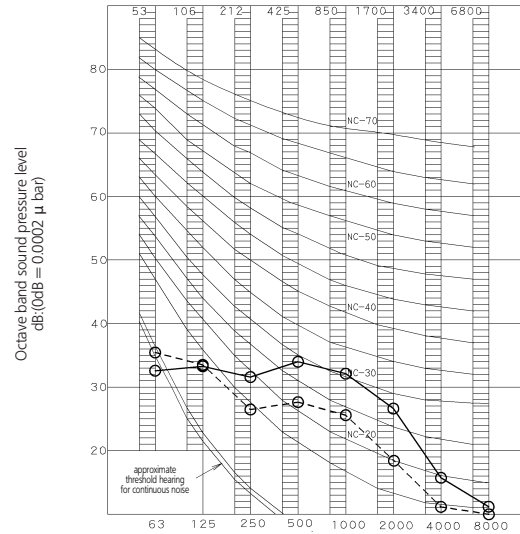
FLXS25B (Heating)
