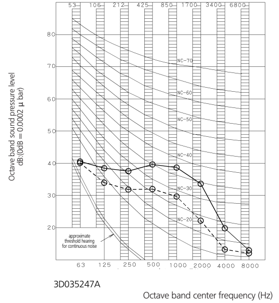
FLXS50B (Heating)
