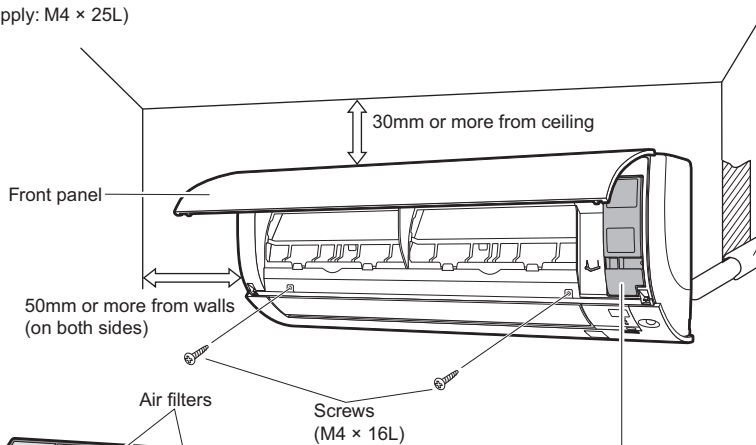
Mounting plate fixing screw (field supply: M4 × 25L)
