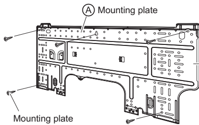
Mounting plate fixing screw (field supply: M4 × 25L)
