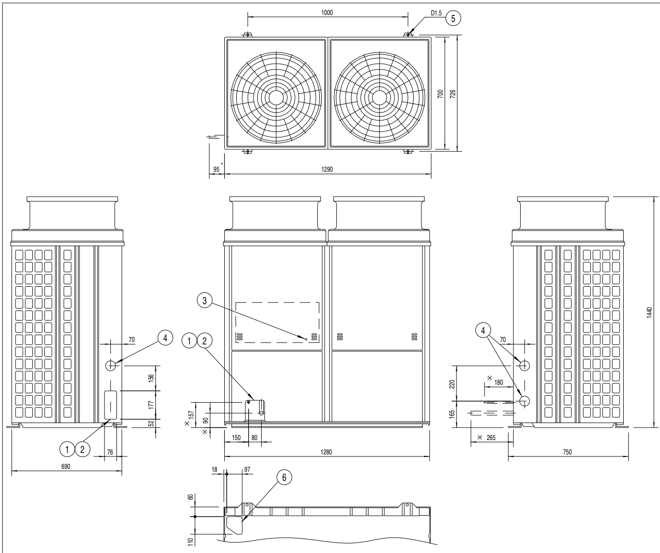
Dimensions marked with x show distances after fixing the connection pipes.
