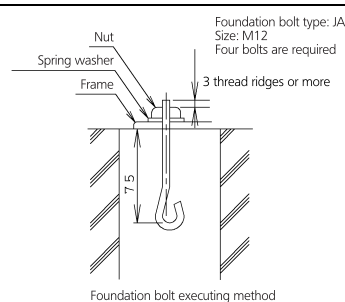
Foundation bolt executing method
