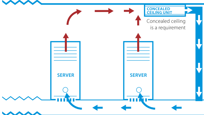
Throughflow racks
